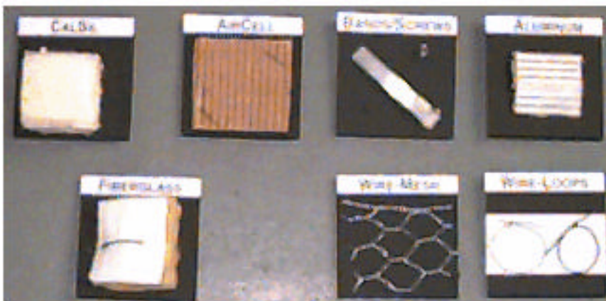
Figure 6. Samples of lagging and insulation materials.
