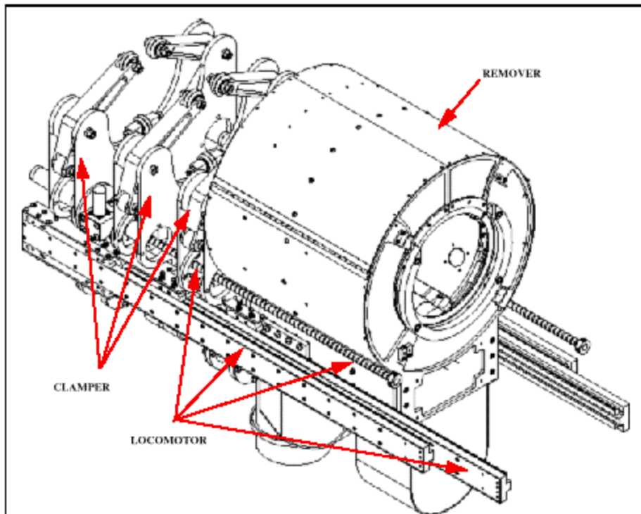
Figure 4. Three-dimensional drawing of the abatement head.
