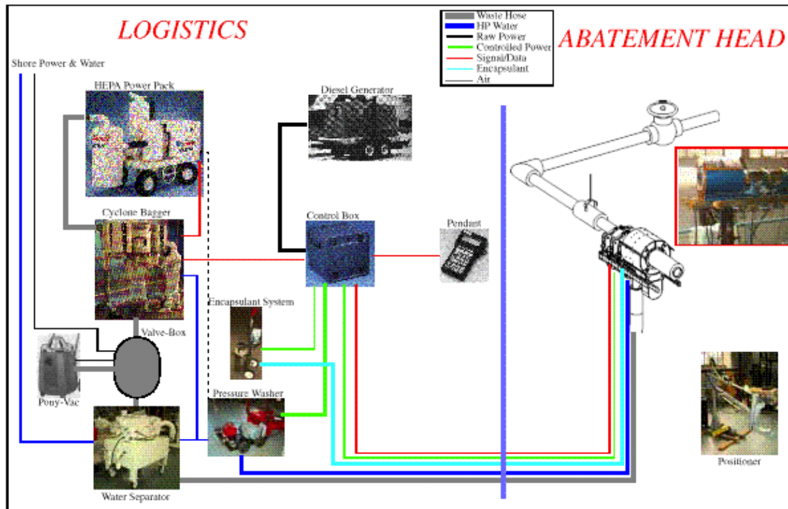
Figure 3. BOA system components and interconnection.
